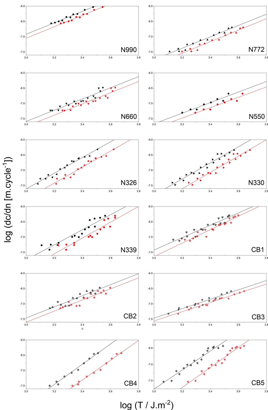
FIG. 6. — Logarithm of fatigue crack growth rate data for each compound plotted versus logarithm of tearing energy. Red data sets are from tearing energies calculated from mechanical loading curves; black data sets are from tearing energies calculated from mechanical unloading curves.
